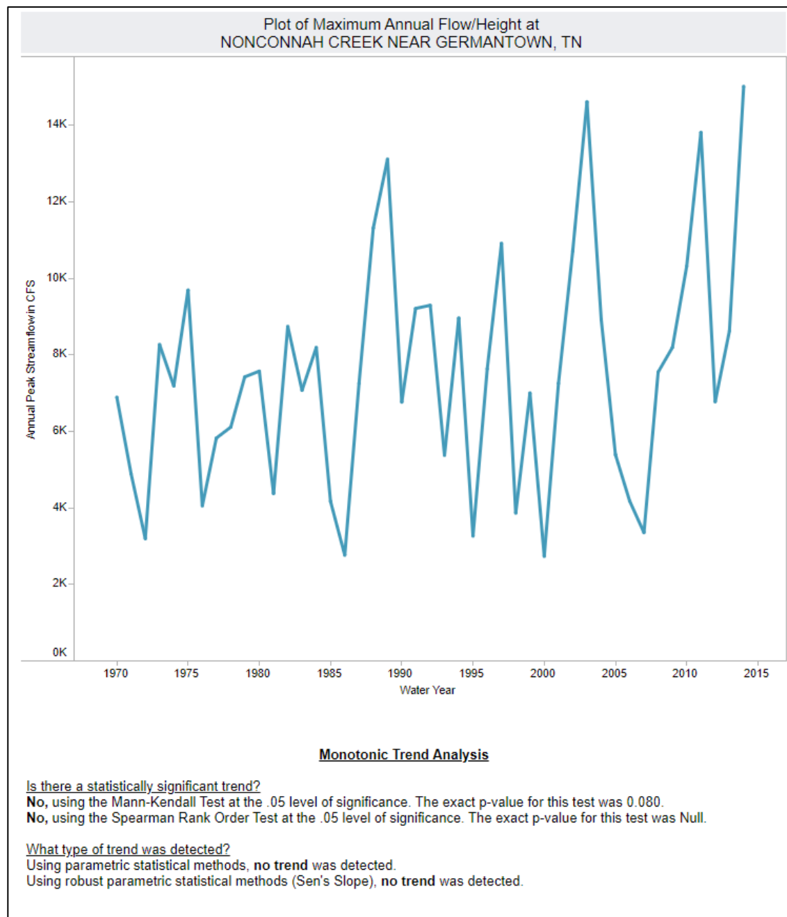
Figure H:1-15. Monotonic Trend Analysis for the full POR (1970-2014), taken from the US Army Corps of Engineers Non-stationarity Detection Tool
