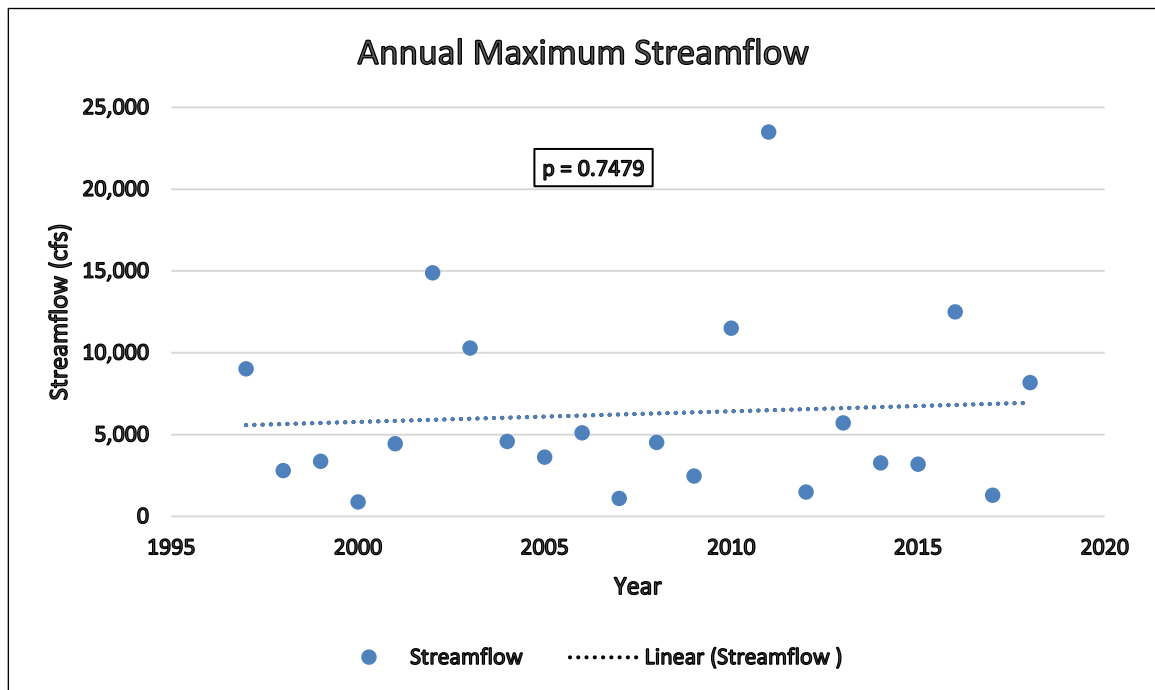
Figure H:1-10. Annual Peak Streamflow at USGS 07275900 Coldwater River near Olive Branch, MS
