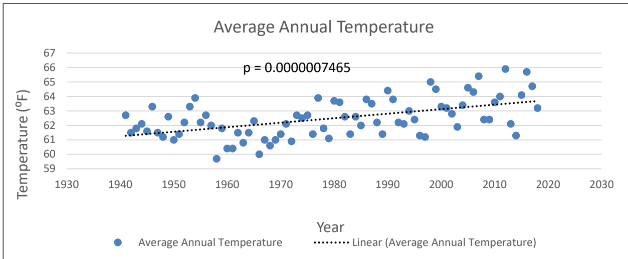
Figure H:1-4. Annual Average Temperature and P-Value from 1940 – 2018 (MEM)
