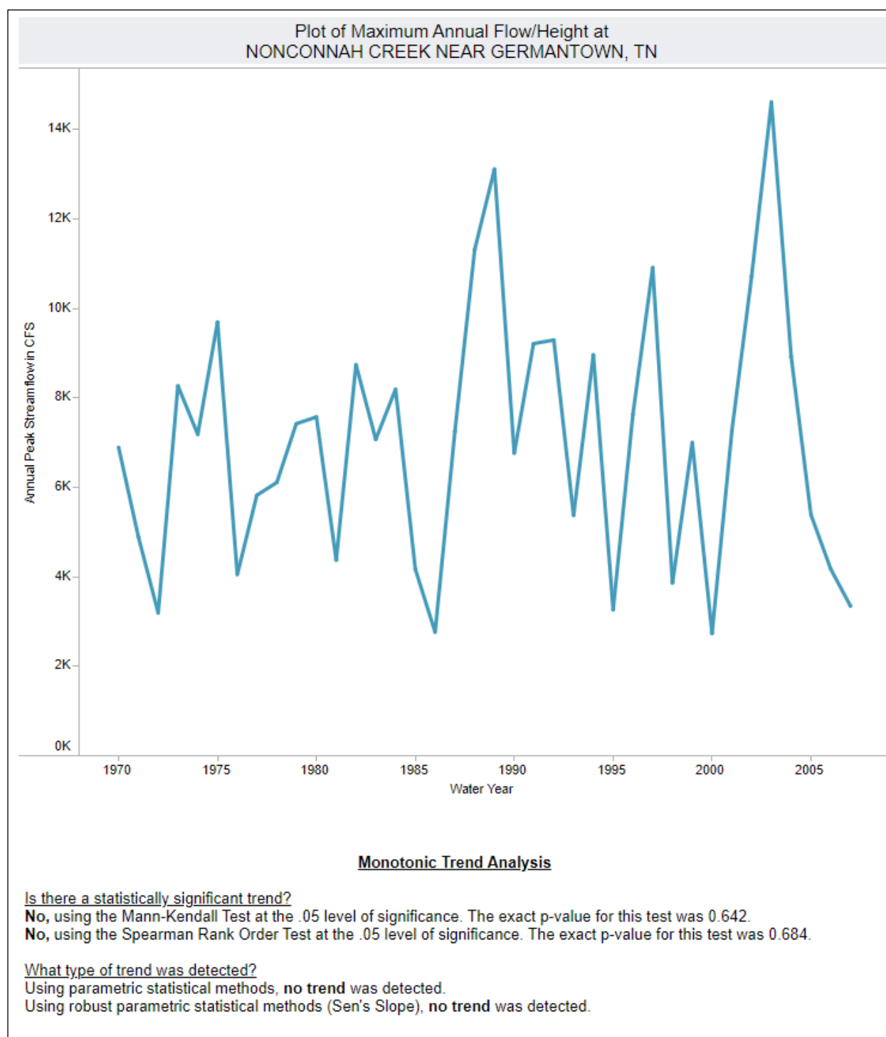
Figure H:1-16. Monotonic Trend Analysis for the POR before the Non-Stationarity (1970-2007), taken from the US Army Corps of Engineers Non-stationarity Detection Tool
