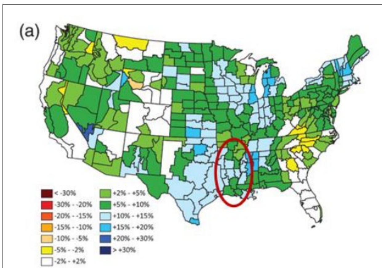
Figure H:1-7. Linear Trends in Annual Precipitation, 1895 - 2009, Percent Change per Century. The Lower Mississippi River Region is within the Red Oval (McRoberts and Nielsen-Gammon, 2011). DeSoto County, where the Horn Lake Creek is located, has Experienced a 10 - 15% Increase in Precipitation over the Century
