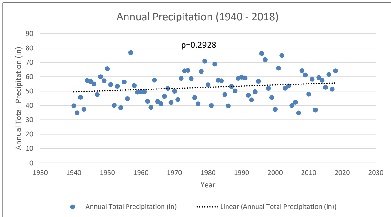
Figure H:1-8. Annual Total Precipitation and P-Value from 1940 – 2018 (MEM)
