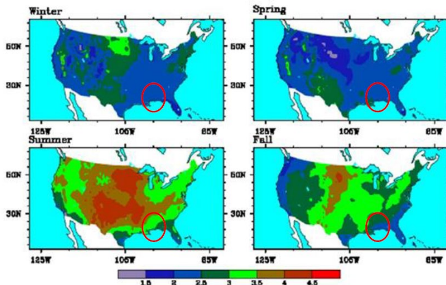
Figure H:1-5: Projected Changes in Seasonal Maximum Air Temperature, °C, 2041 – 2070 vs. 1971 – 2000. The Lower Mississippi River Region is within the Red Oval. (Liu et al., 2013 reprinted from USACE, 2015)
