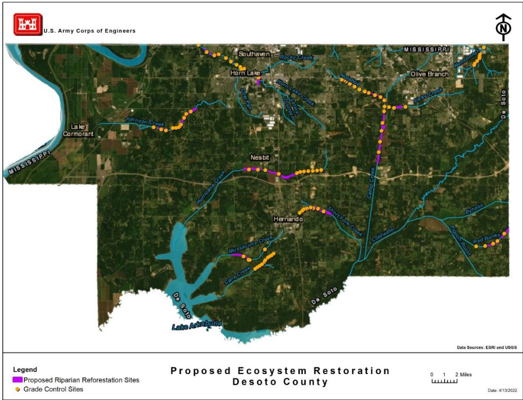
Figure H:1-2. Ecosystem Restoration Tentatively Selected Plan
