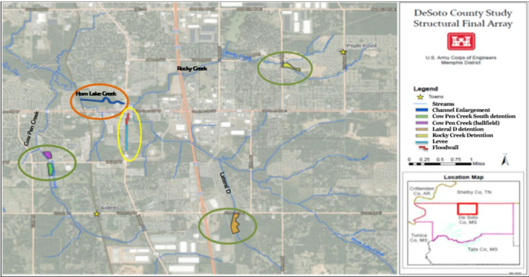
Figure H:1-1. FRM Structural Final Array
