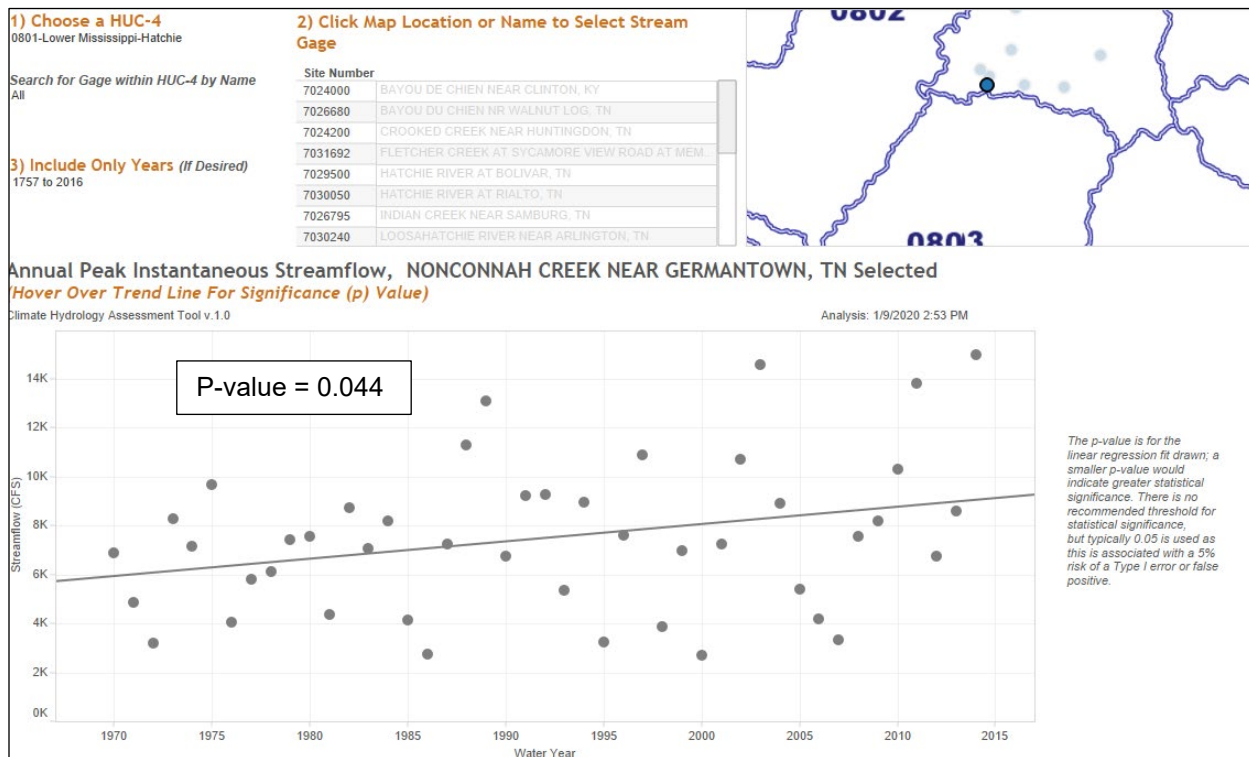
Figure H:1-17. CHAT Output for USGS 07032200 for Nonconnah Creek near Germantown, TN, P-Value=0.044
